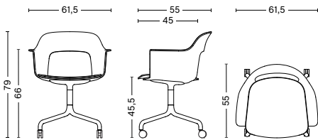
LAYOUT ARMCHAIR 262 Width 61,5 cm Depth 55 cm Height 79 cm Seat height 45,5 cm Armrest height 66 cm Weight 9,5 kg
