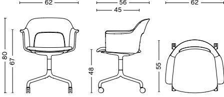
LAYOUT ARMCHAIR 264 Width 62 cm Depth 56 cm Height 80 cm Seat height 48 cm Armrest height 67 cm Weight 10,9 kg
