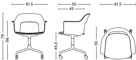
LAYOUT ARMCHAIR 261 Width 61,5 cm Depth 55 cm Height 79 cm Seat height 45,5 cm Armrest height 66 cm Weight 9,7 kg
